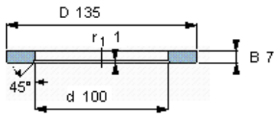
Universal washer
